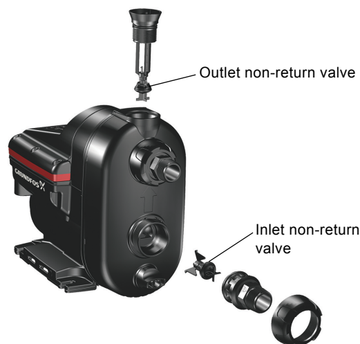
Fig. 19 Outlet and inlet non-return valves
