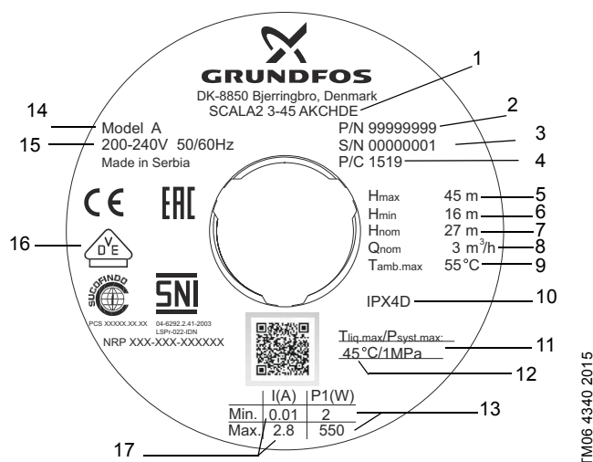
Fig. 11 Example of nameplate
